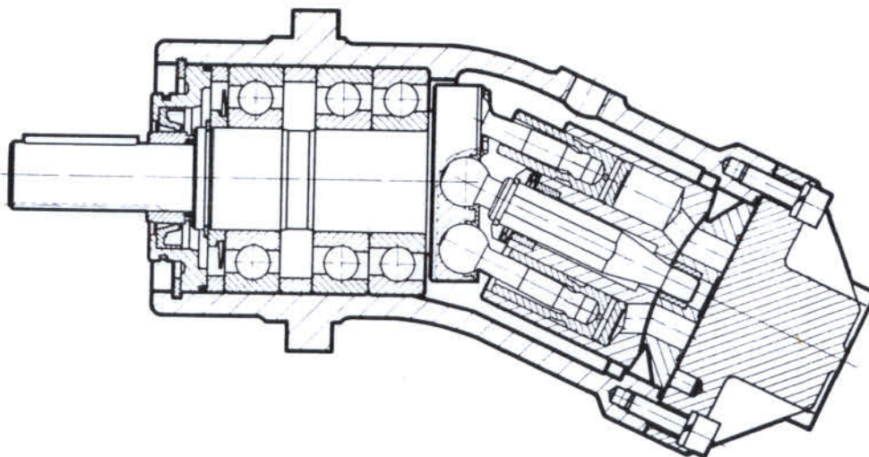
FIXED DISPLACEMENT UNIT
